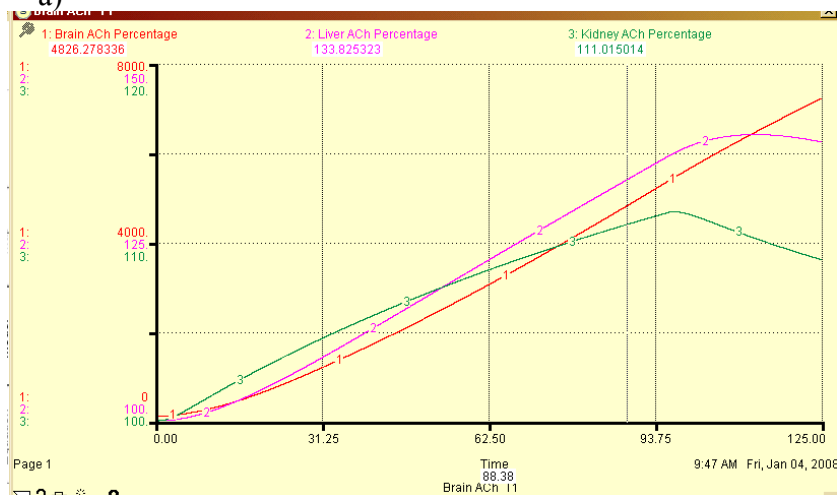
Figure 22. Figure a demonstrates the building up of ACh in three tissue groups from an inhalation exposure. The levels of ACh are measured at 60 minutes. Figure b shows the same tissues when the body is exposed to a dermal exposure. As can be seen it takes 88 minutes of exposure for all of the tissues to at least equal the inhalation exposure.
